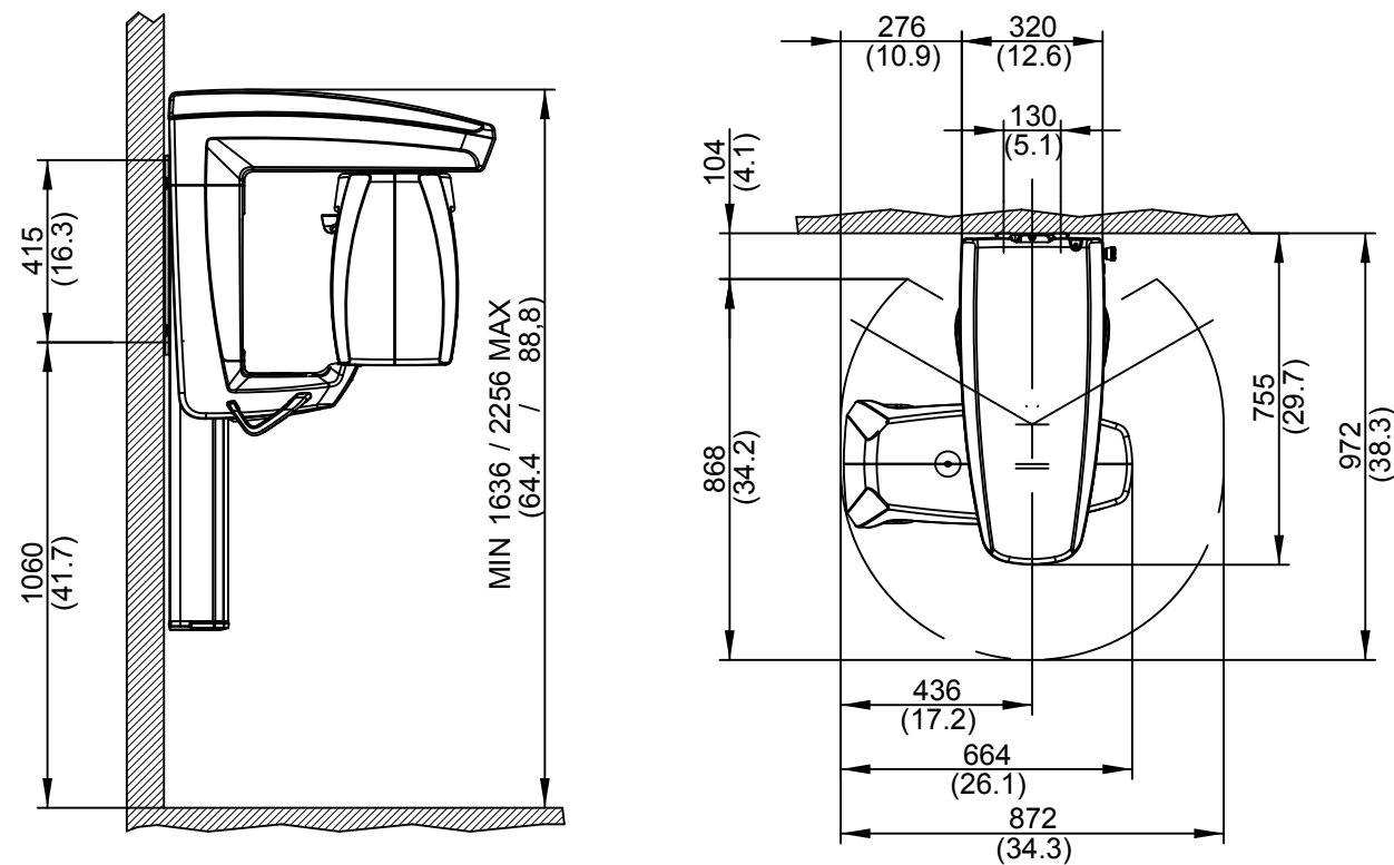
WALL-MOUNTED VERSION
