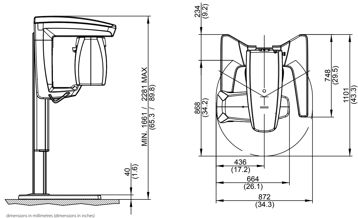
FREE-STAND FLOOR-MOUNTED VERSION
